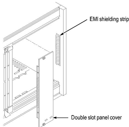
Figure 5: Installing panel covers on the benchtop mainframe
