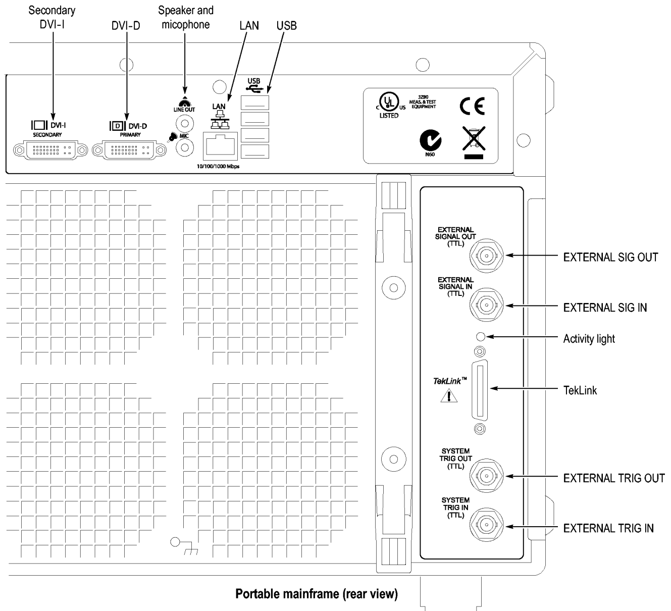
Figure 6: TLA7012 accessories connections
