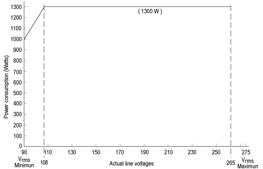
Figure 1: Maximum power allowed to modules at various line voltages for TLA7016 mainframes serial number B020000 and higher
