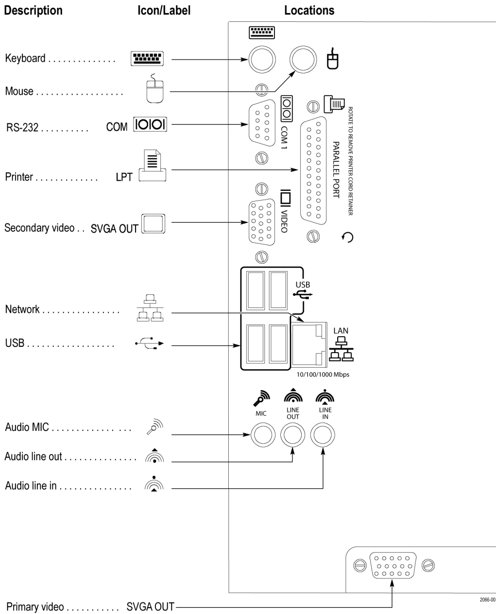
Figure 9: TLA5200B accessory connections
